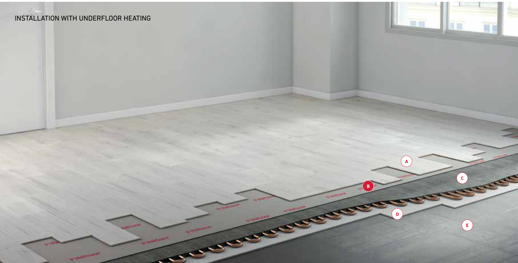
A FINFLOOR B FINFLOOR SILENT ELITE UNDERLAY C UNDERFLOOR HEATING D INSULATION E SUB-FLOOR
